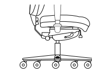
XC Extended Seat Height 19½" - 26¾" -2¼" for OT mechanism, no SS.
